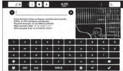
Coordinate Search
