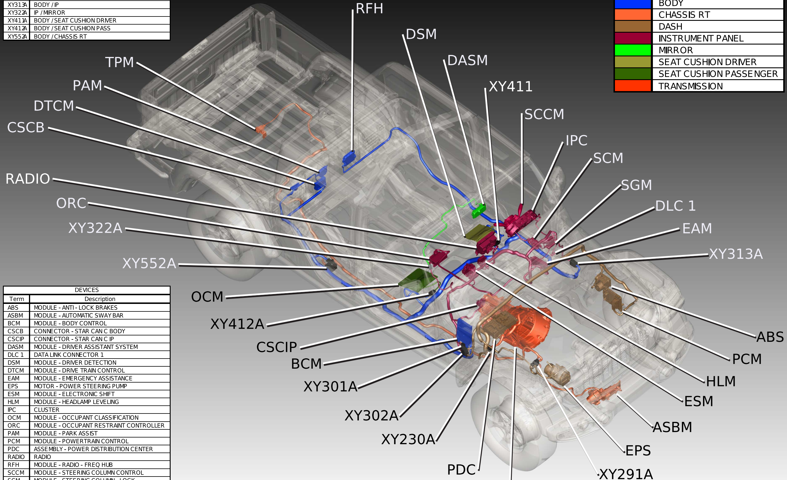
CAN C Network Topology
