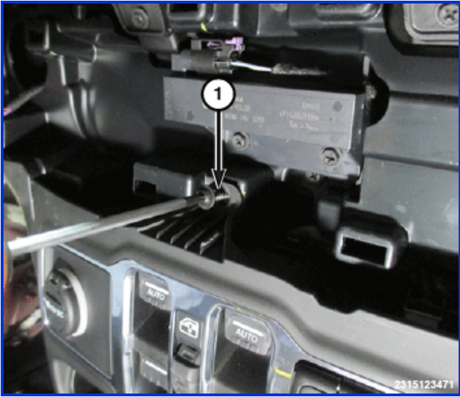
1 - Screw
