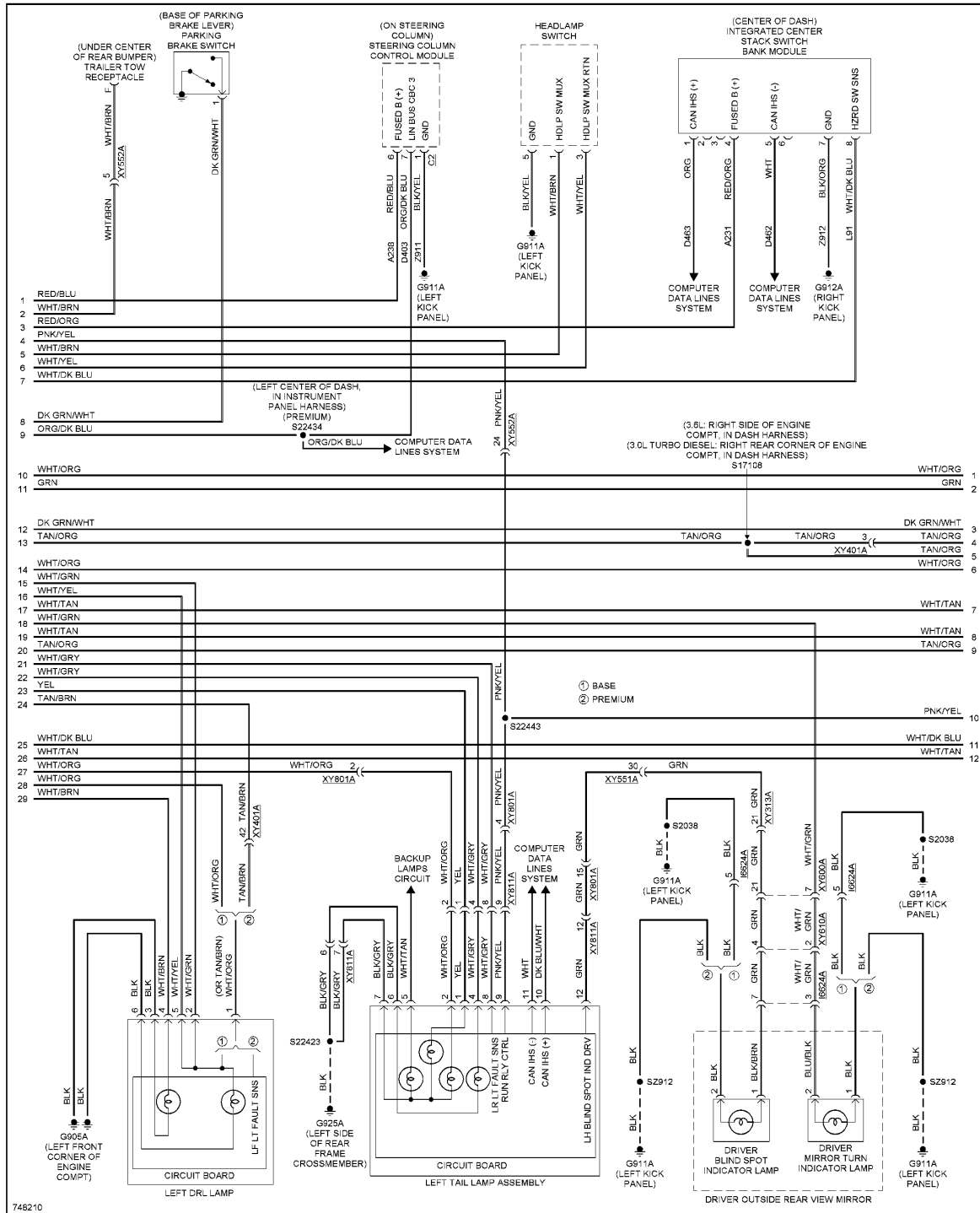
Fig. 43: Exterior Lamps Circuit (2 of 3)
