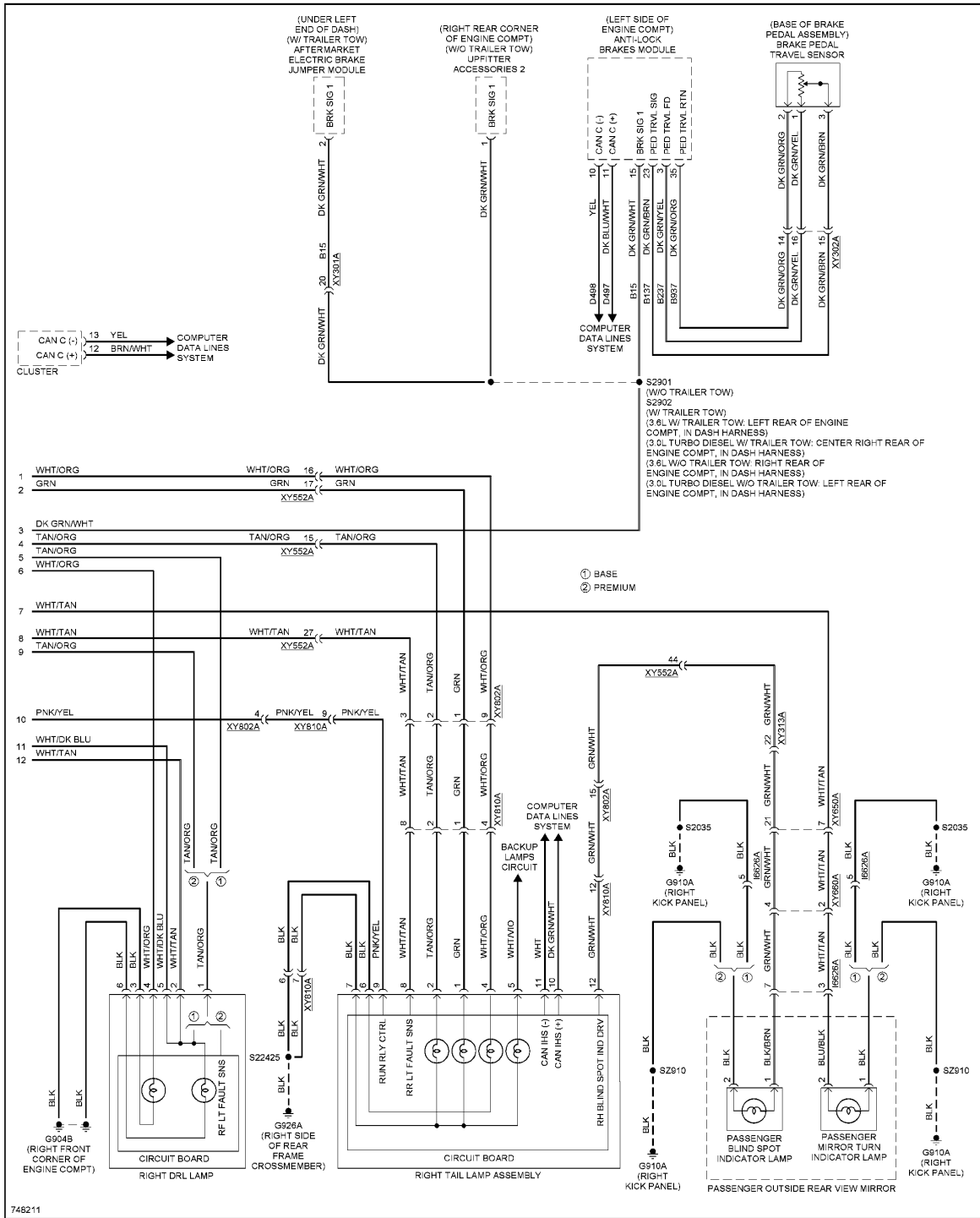
Fig. 44: Exterior Lamps Circuit (3 of 3)
