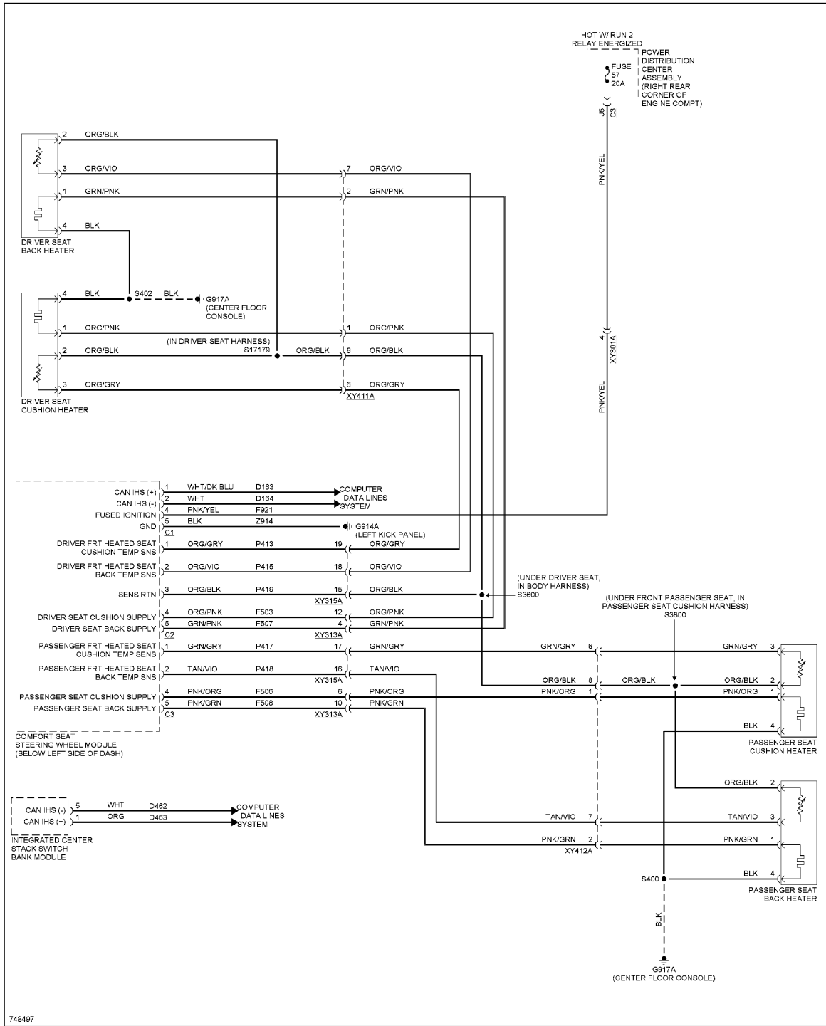
Fig. 75: Heated Seats Circuit
