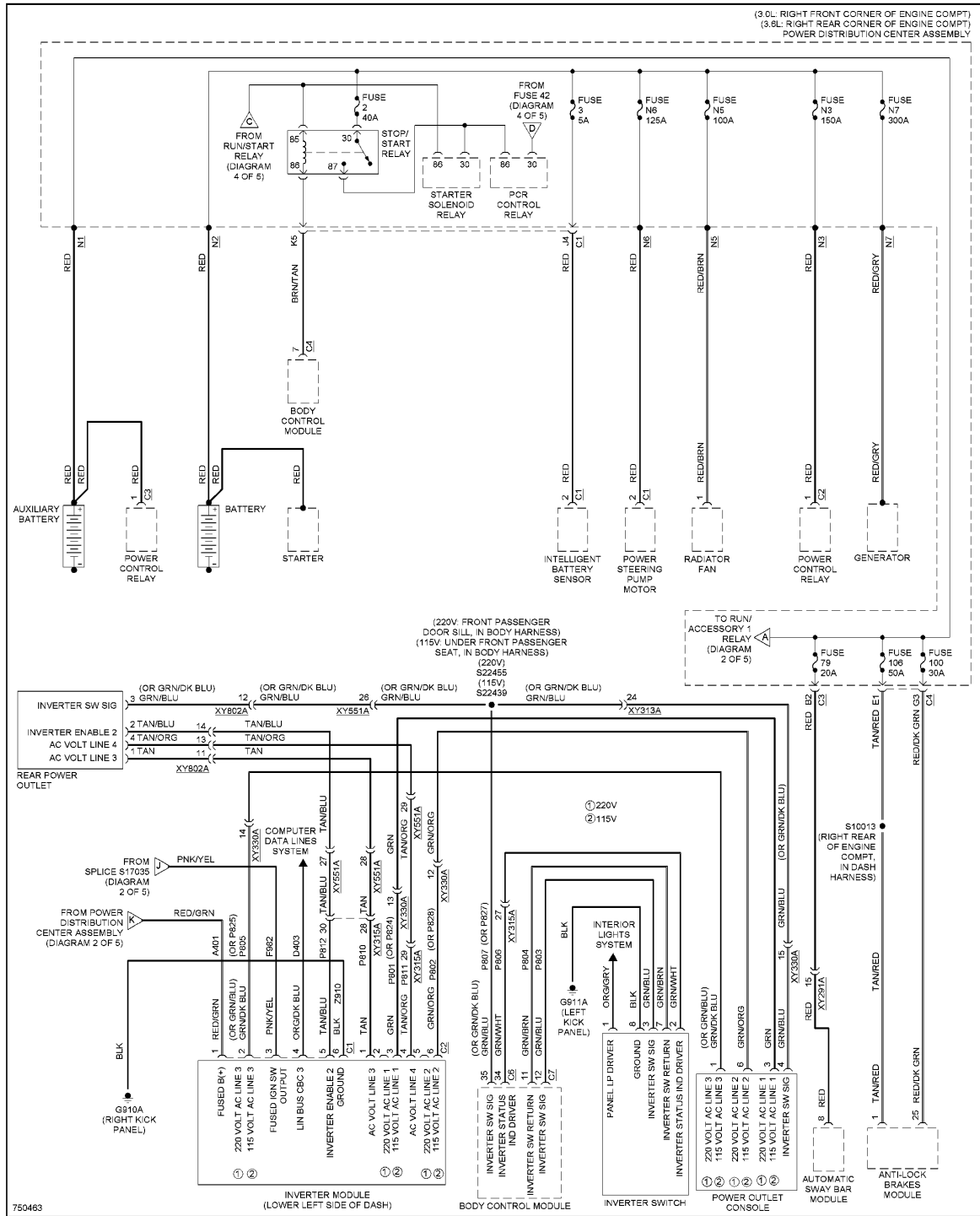
Fig. 65: Power Distribution Circuit (1 of 5)
