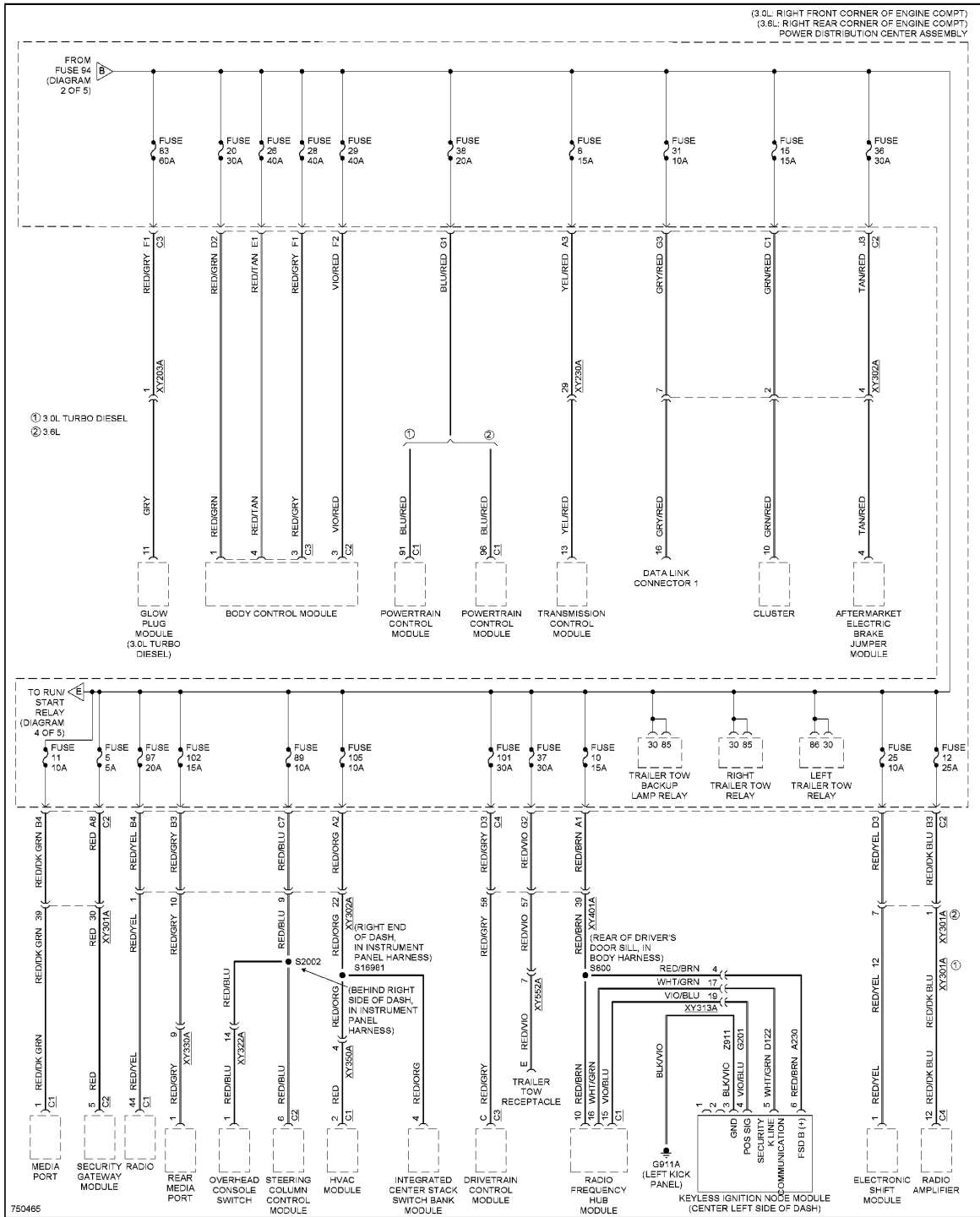
Fig. 67: Power Distribution Circuit (3 of 5)
