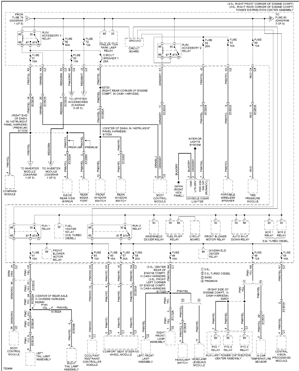
Fig. 66: Power Distribution Circuit (2 of 5)
