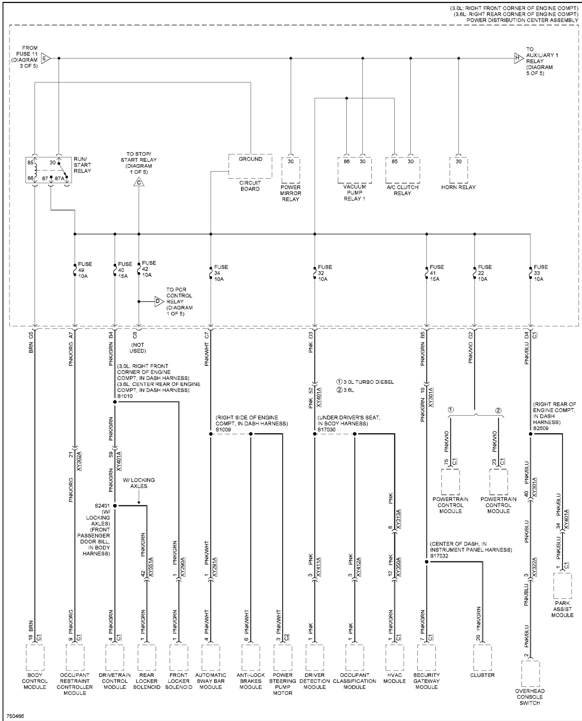
Fig. 68: Power Distribution Circuit (4 of 5)
