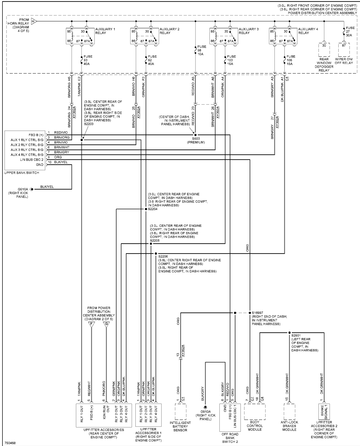
Fig. 69: Power Distribution Circuit (5 of 5)
