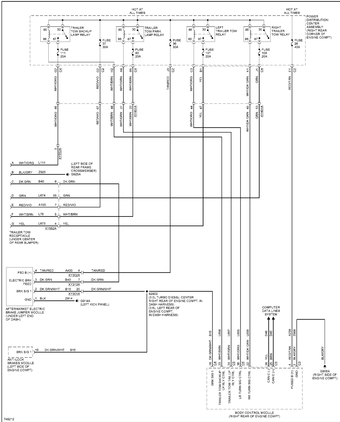
Fig. 45: Trailer Tow Circuit
